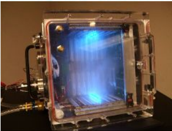
Figure 3 Enclosure with acrylic lid
