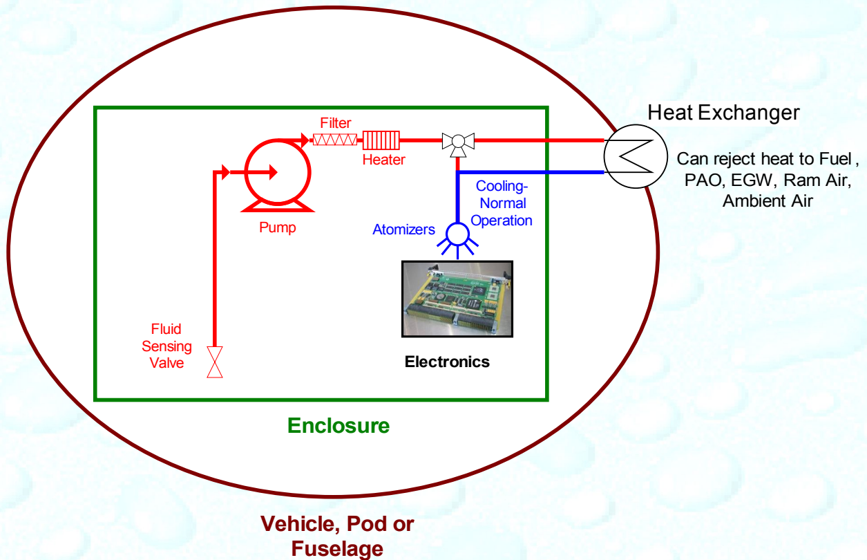
Figure 1 System diagram of direct spray enclosure
